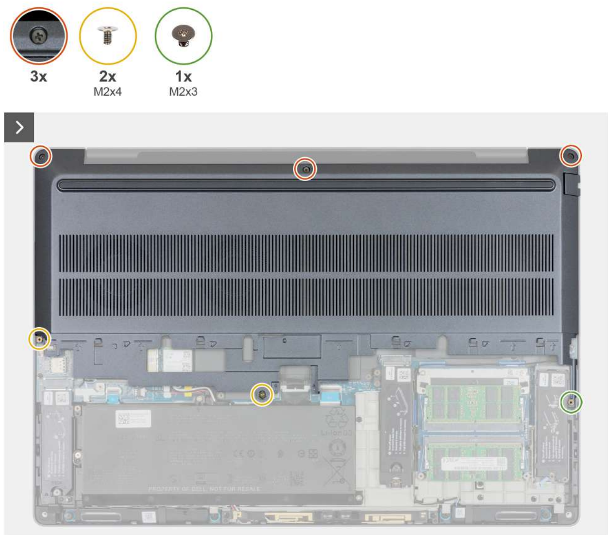
Figure 18. Loosening the three captive screws and removing the three screws
