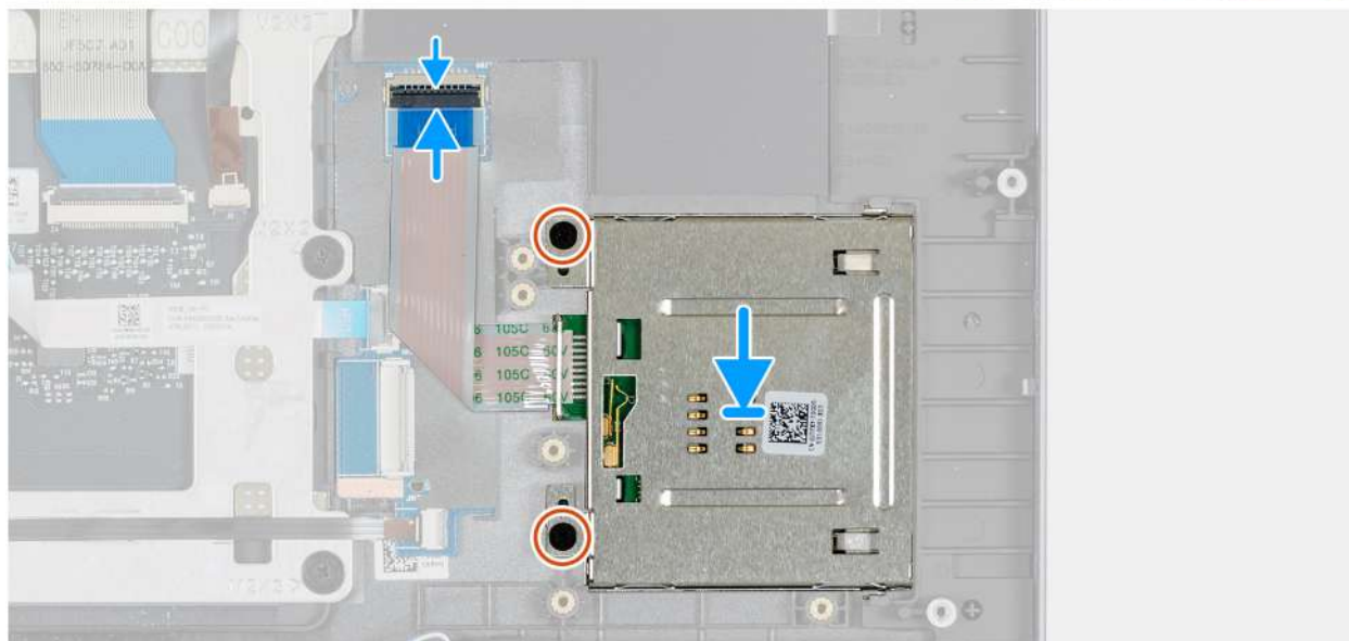
Figure 124. Installing the smart card reader
