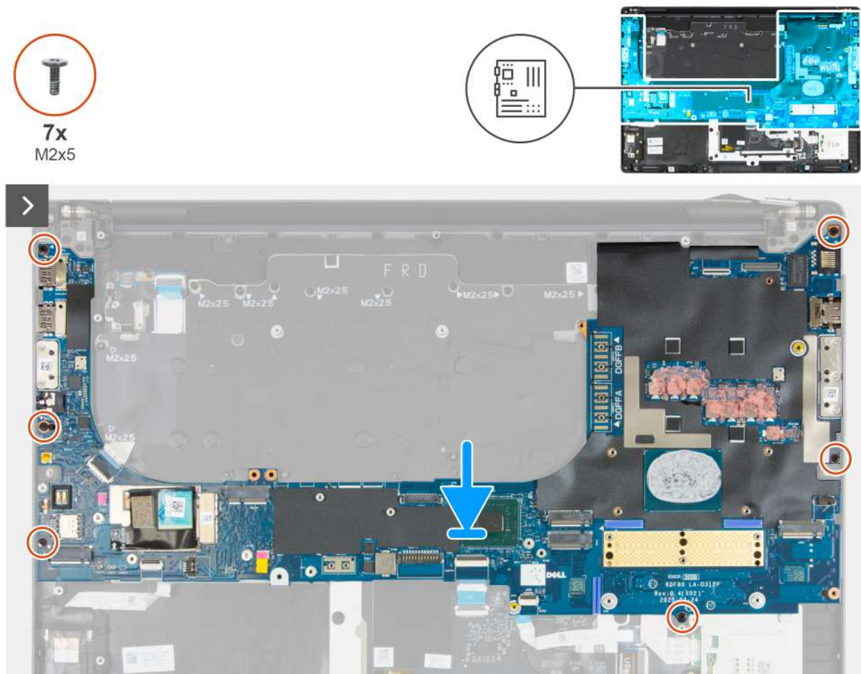
Figure 113. Installing the system board
