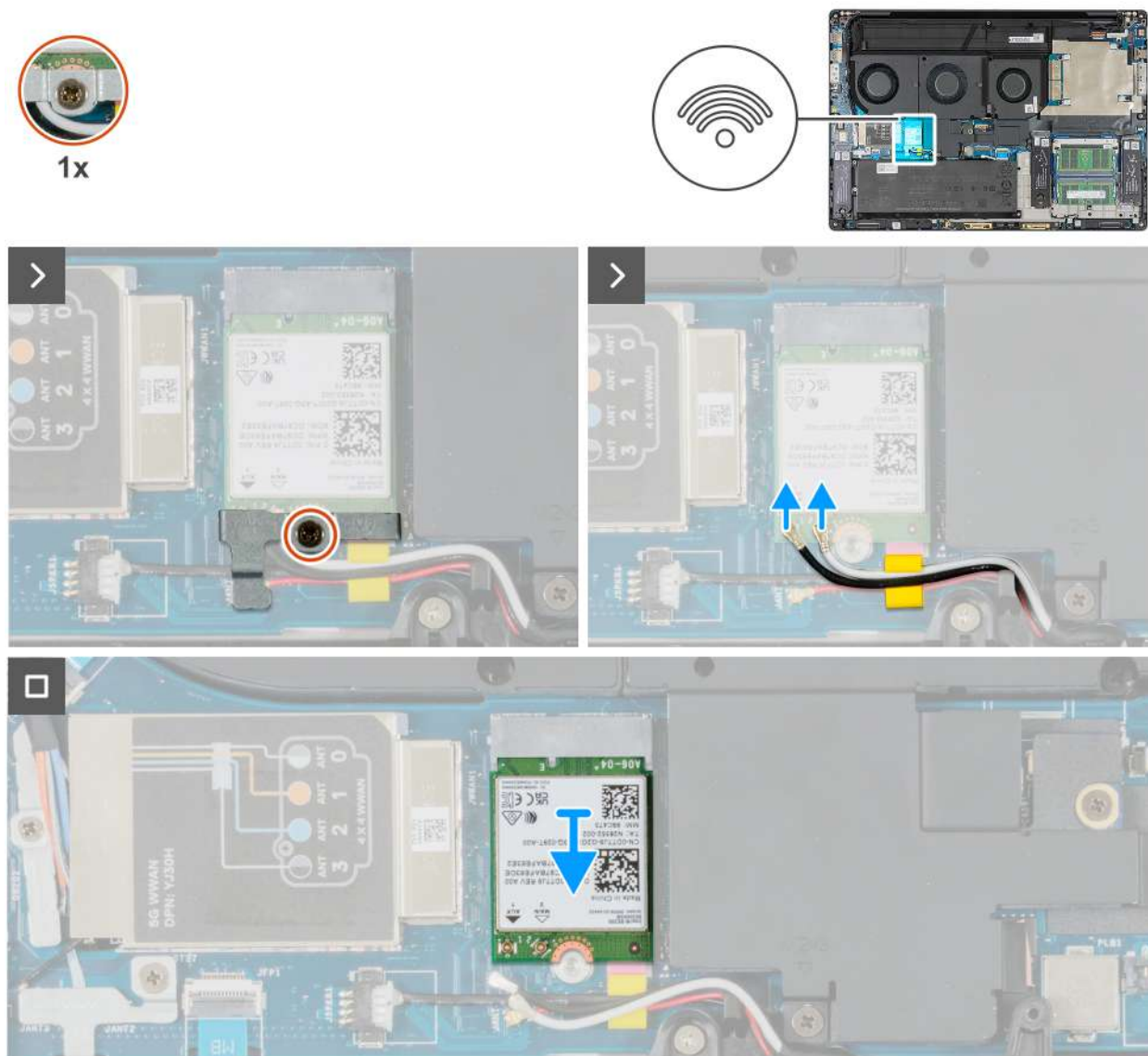
Figure 48. Removing the WLAN card
