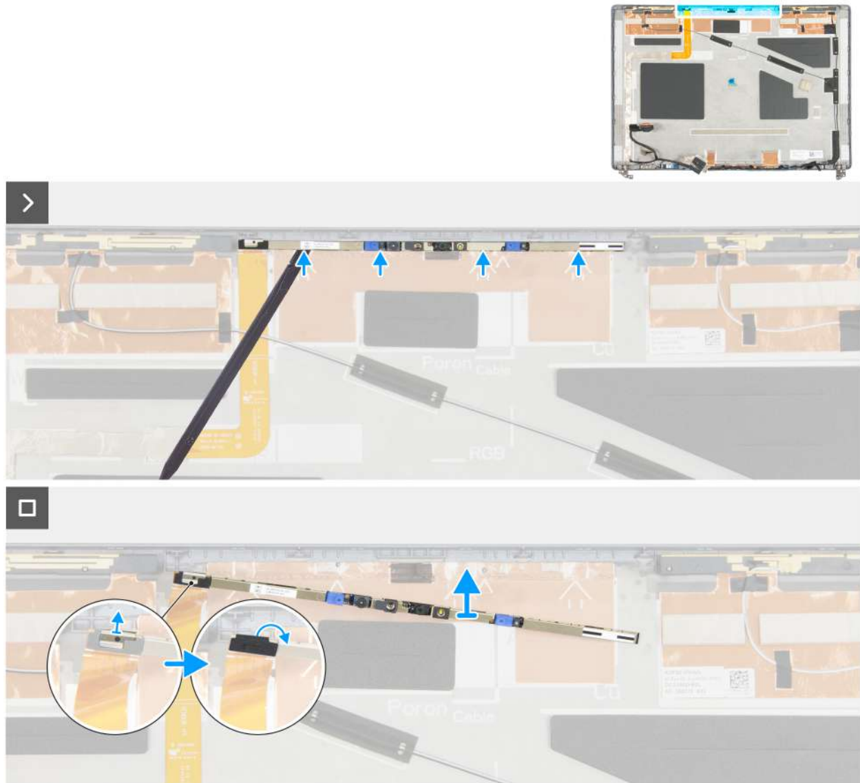
Figure 103. Removing the camera module
