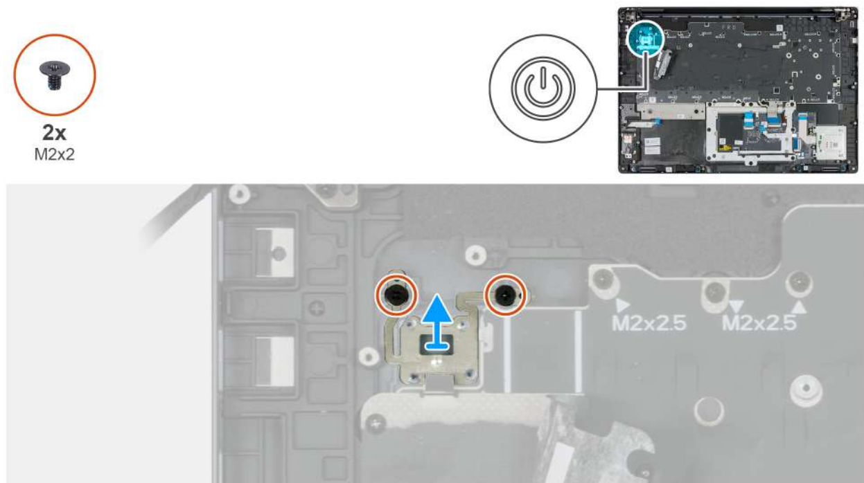
Figure 129. Removing the power button
