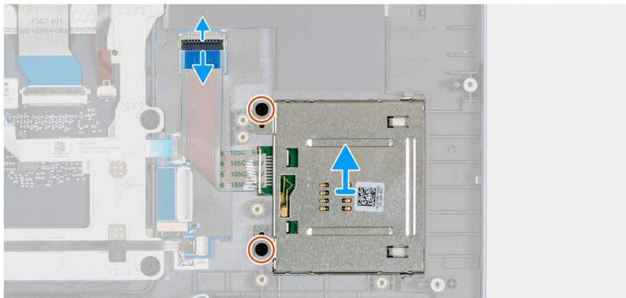
Figure 123. Removing the smart card reader
