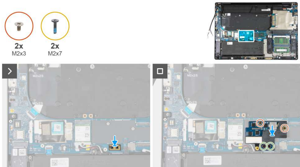
Figure 72. Installing the power board
