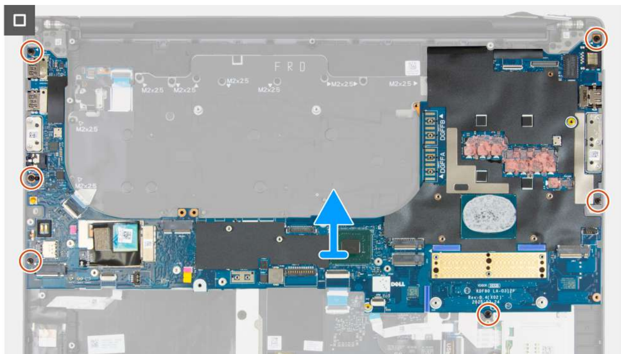
Figure 110. Removing the system board
