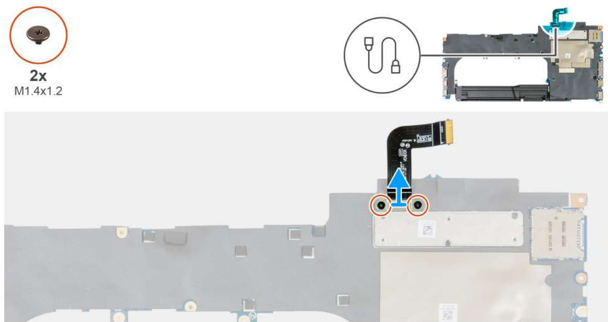
Figure 117. Removing the USH board cable
