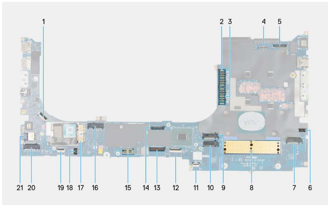
Figure 112. System-board components
