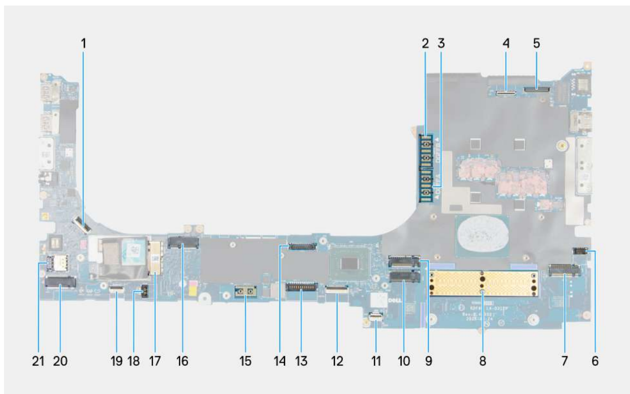
Figure 108. System-board components
