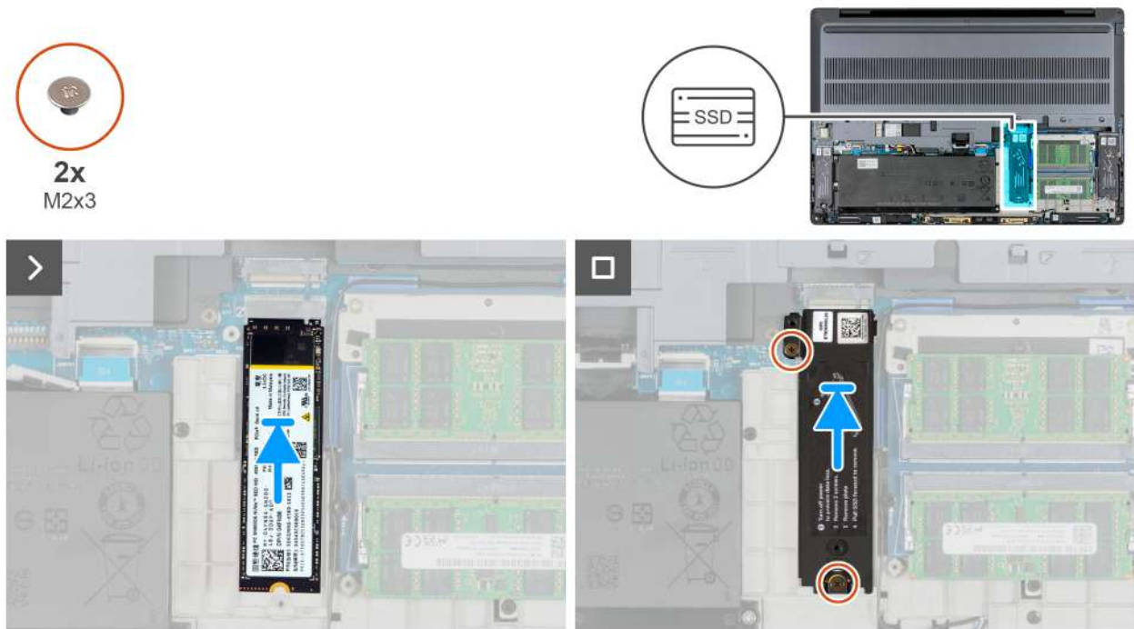
Figure 39. Installing the M.2 2280 SSD in slot 2 (SSD2)
