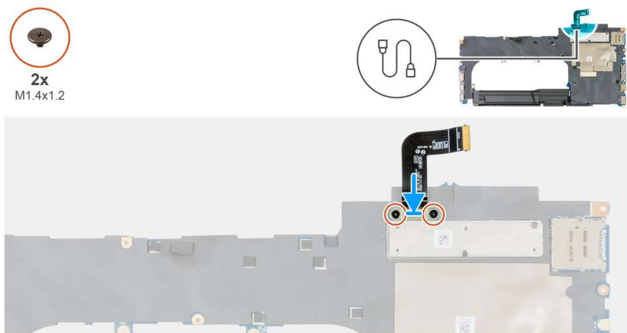
Figure 118. Installing the USH board cable
