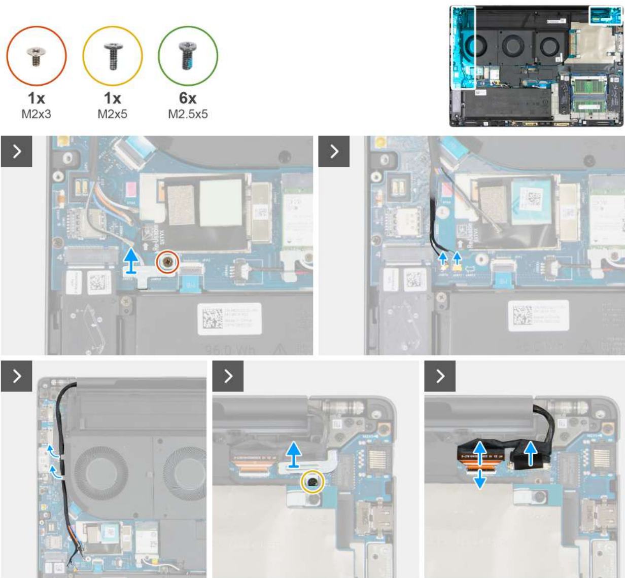
Figure 63. Removing the display assembly
