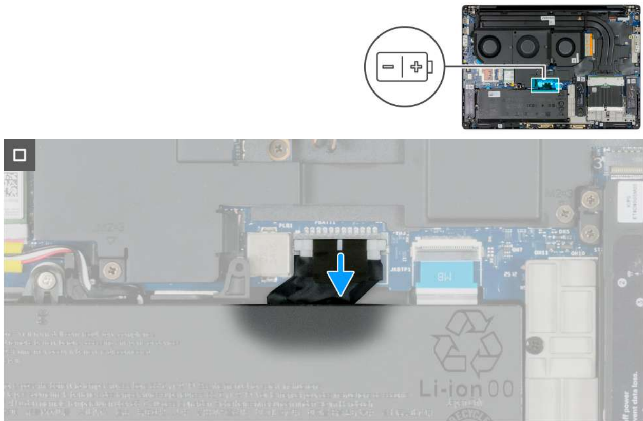
Figure 26. Disconnecting the battery cable
