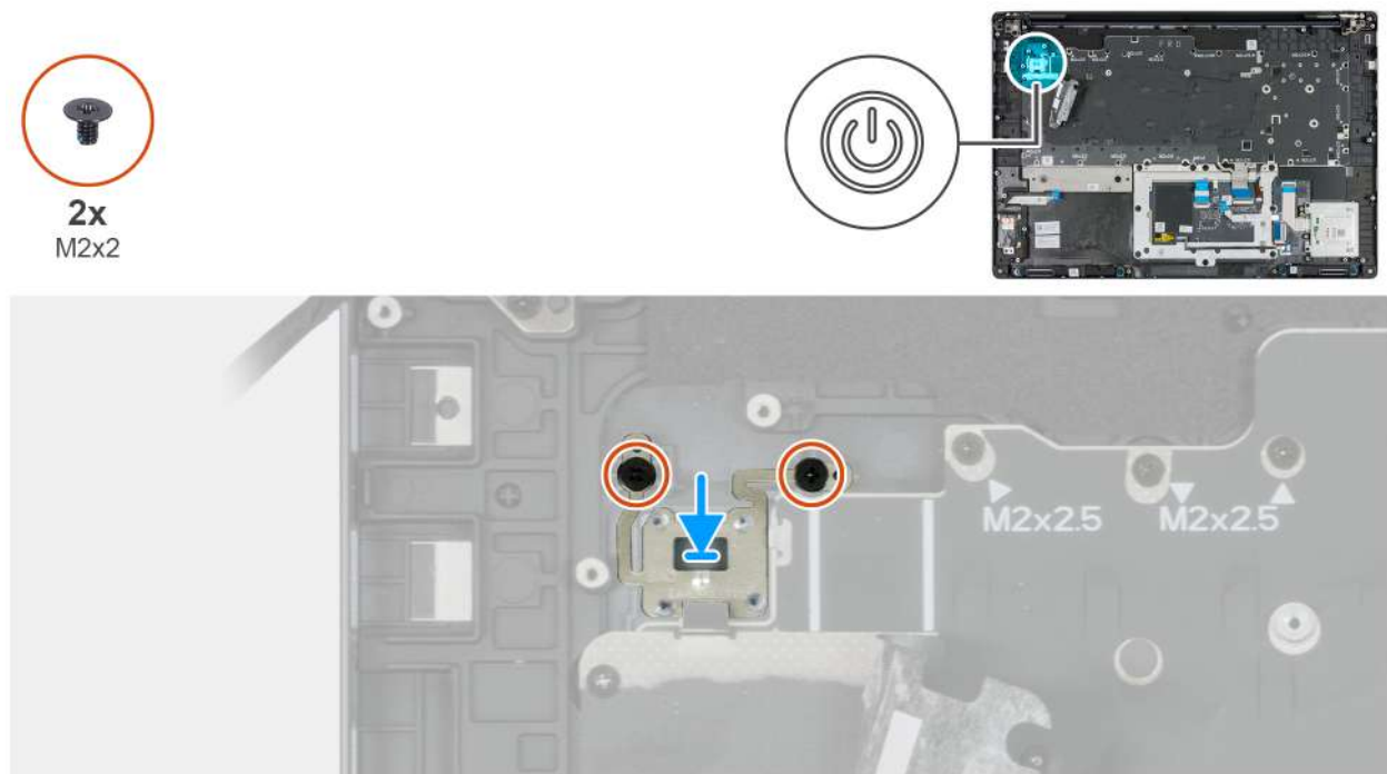
Figure 130. Installing the power button
