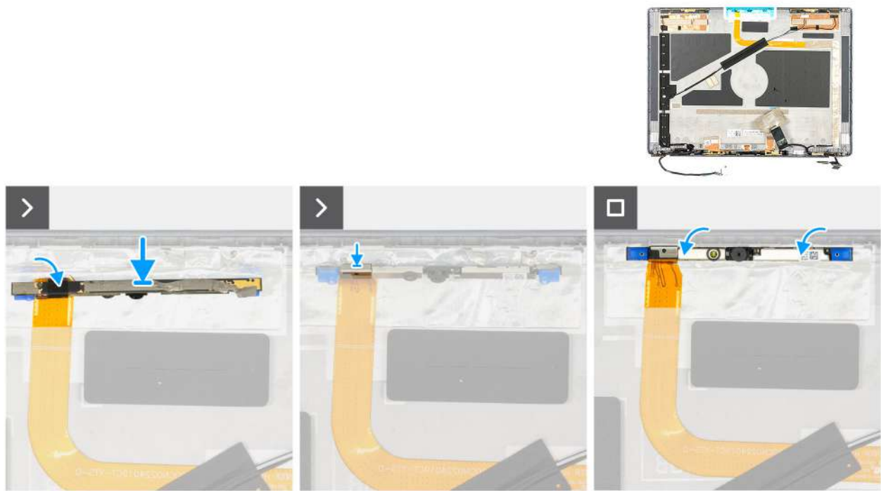
Figure 104. Installing the camera module
