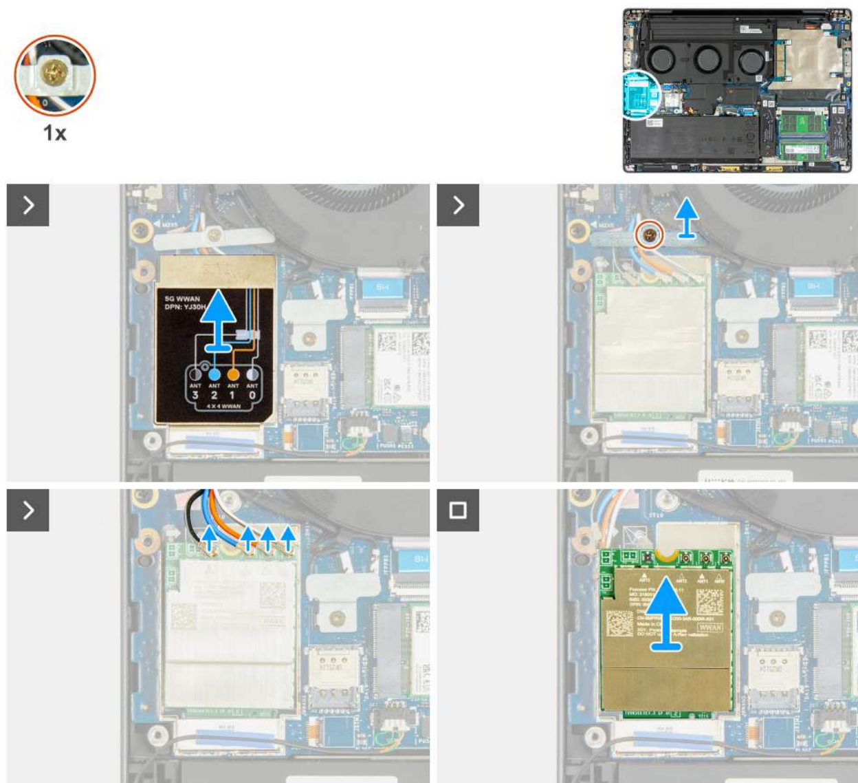
Figure 50. Removing the WWAN card
