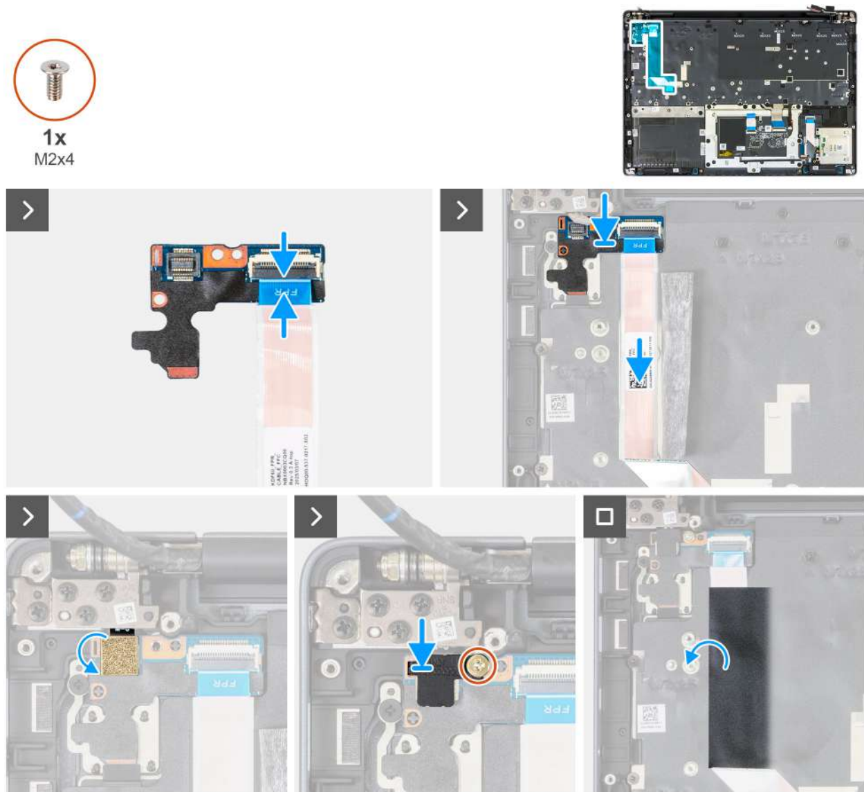
Figure 128. Installing the power button board
