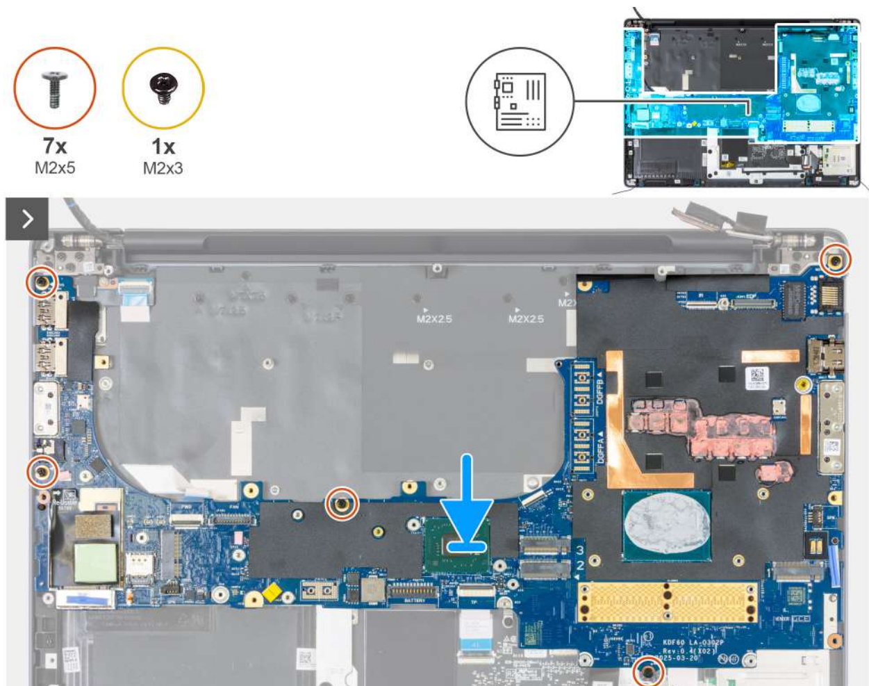
Figure 115. Installing the system board
