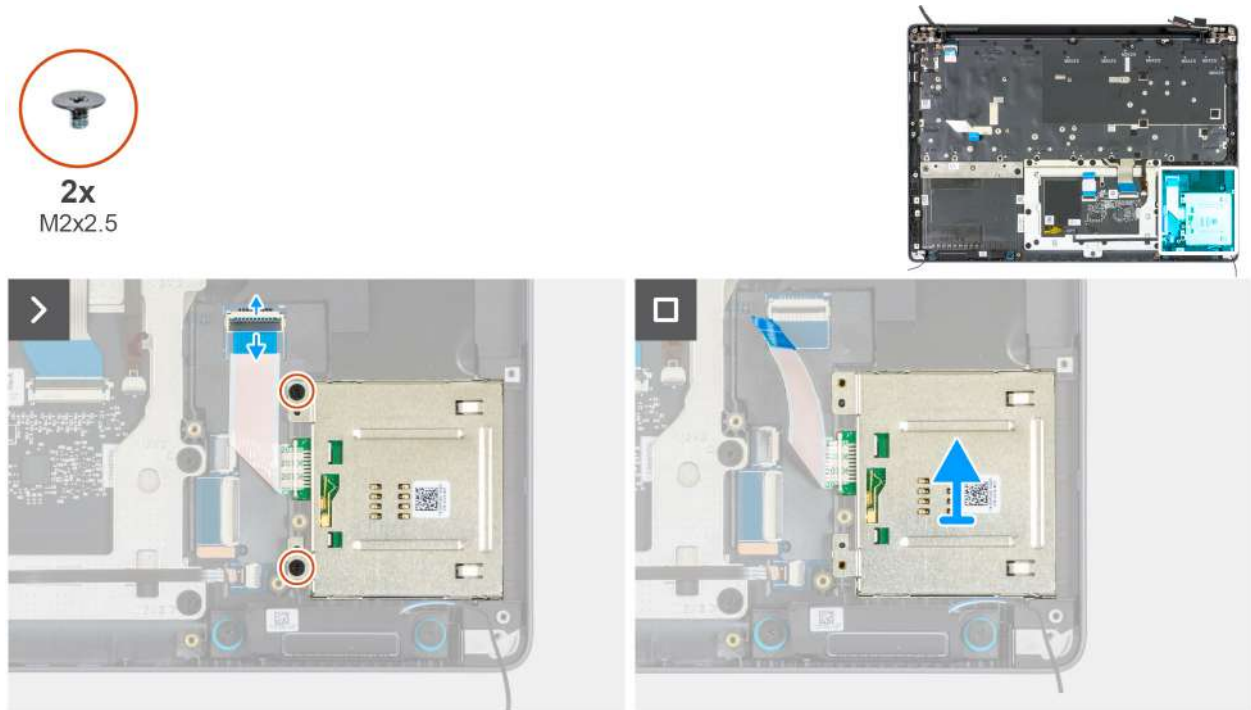
Figure 123. Removing the smart card reader
