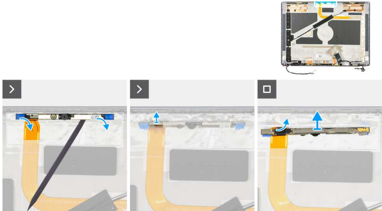
Figure 103. Removing the camera module
