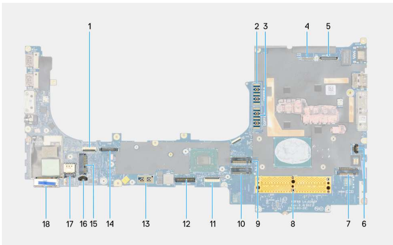
Figure 110. System-board components
