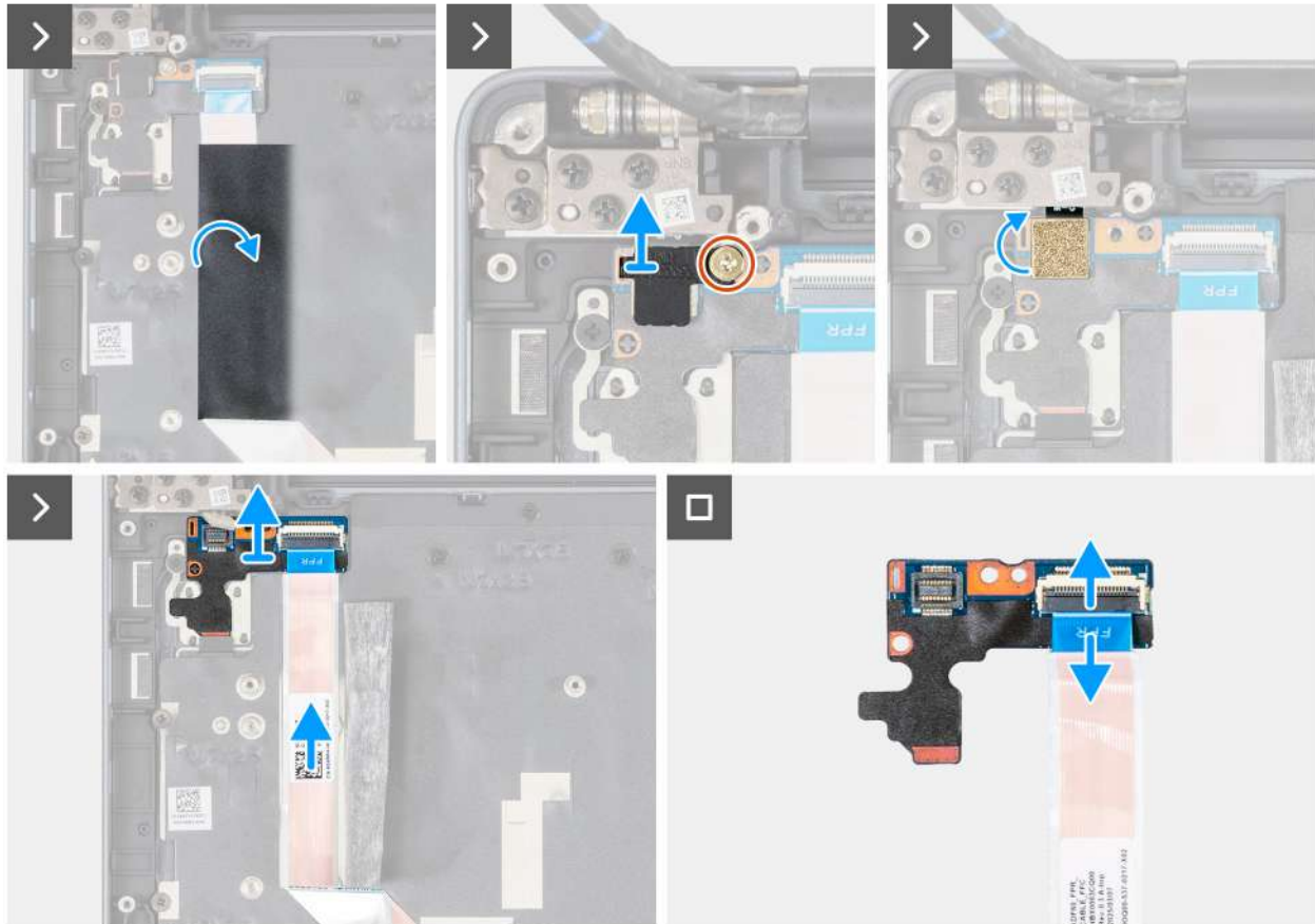
Figure 127. Removing the power button board
