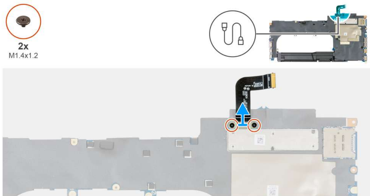
Figure 119. Removing the USH board cable
