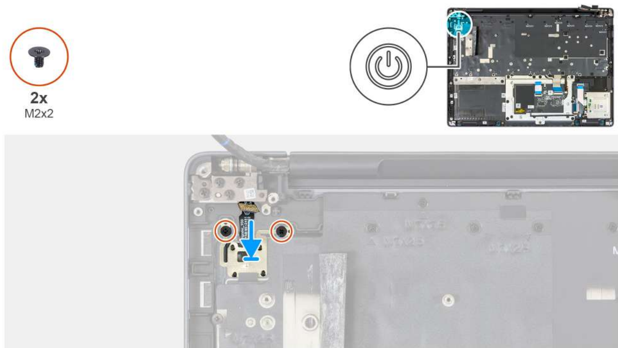
Figure 130. Installing the power button
