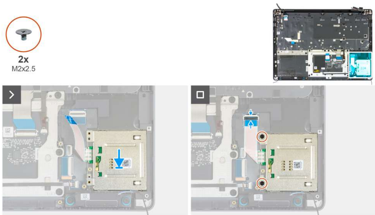
Figure 124. Installing the smart card reader
