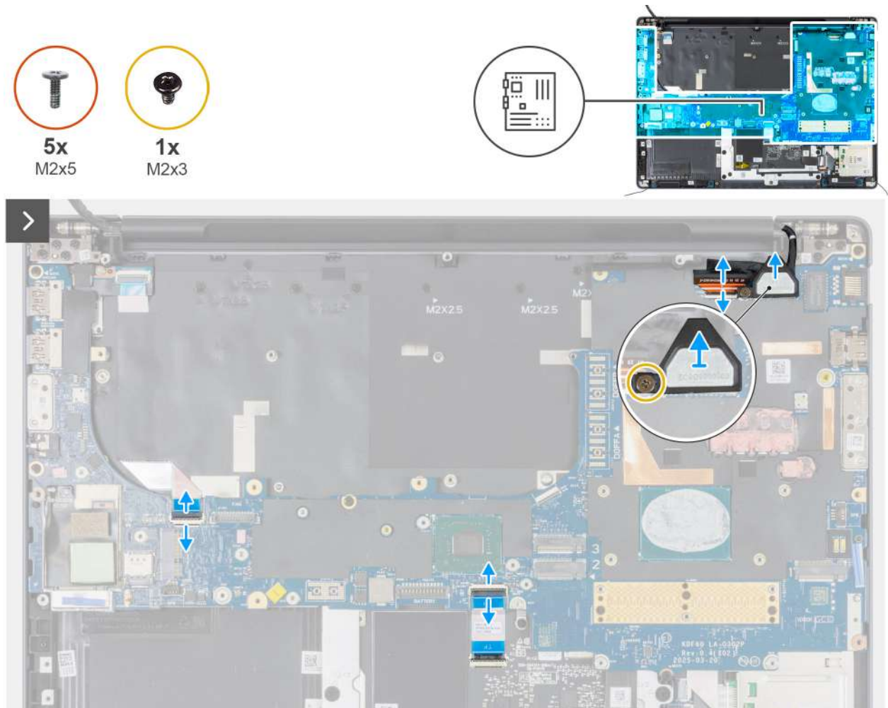
Figure 111. Removing the system board
