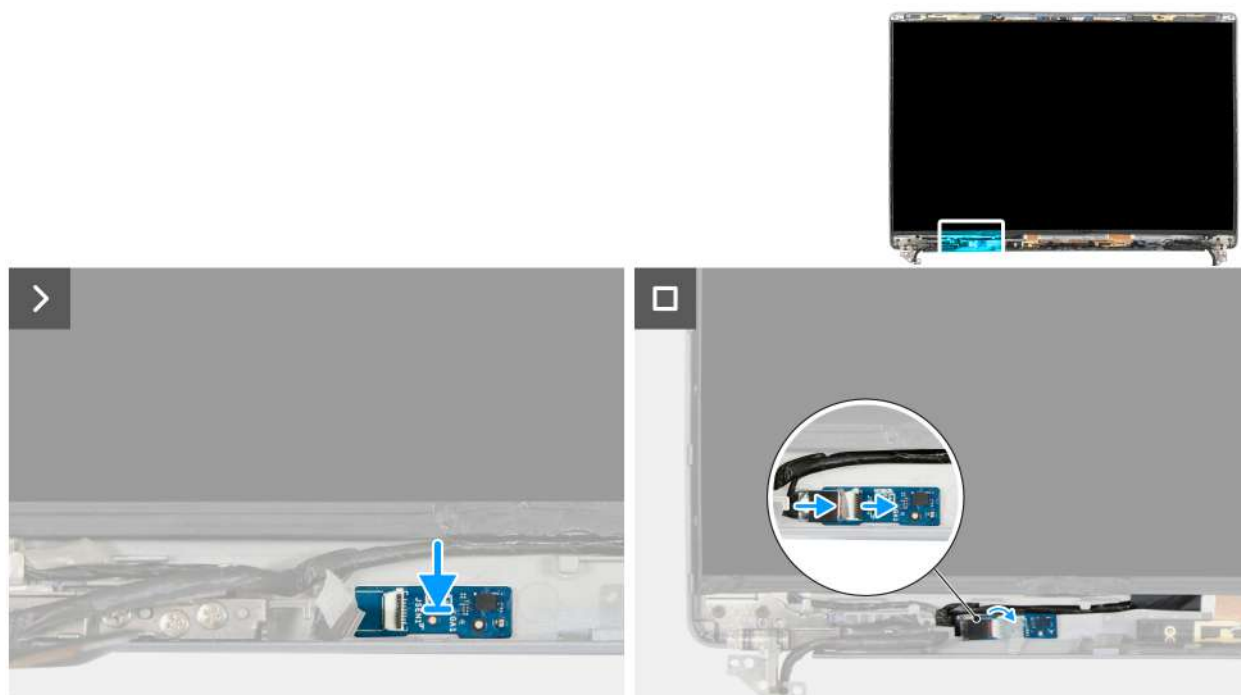
Figure 102. Installing the sensor board
