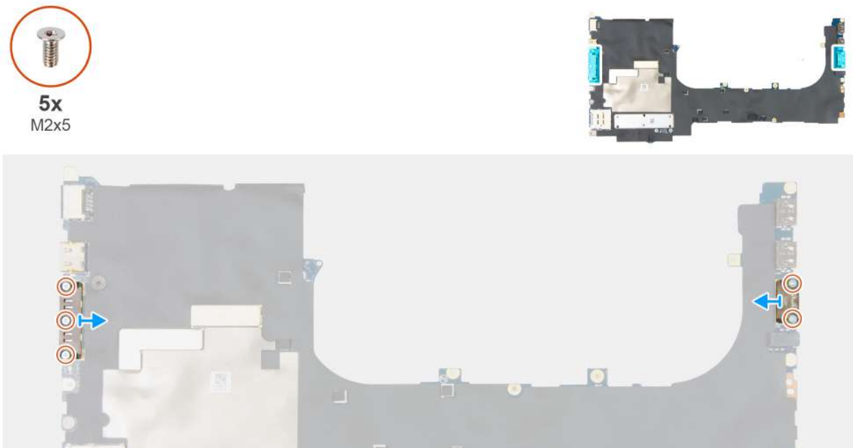
Figure 117. Removing the USB Type-C connector module
