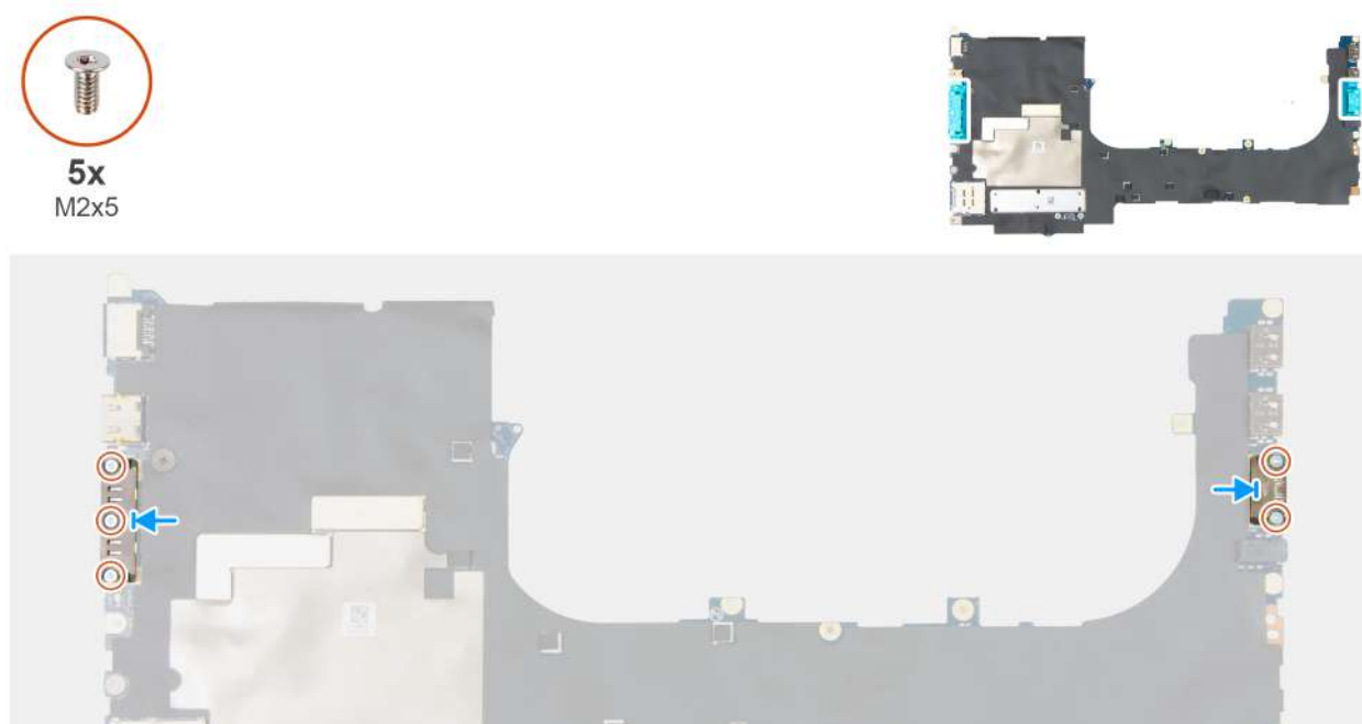
Figure 118. Installing the USB Type-C connector module
